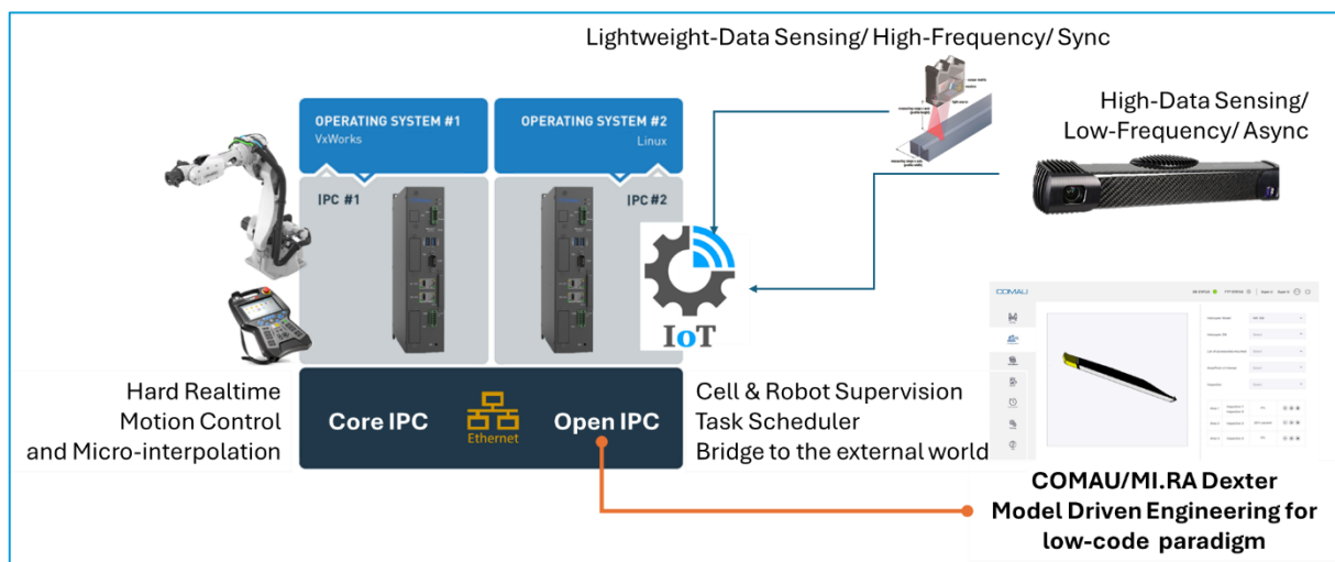
Figure 1 The Architecture for the new generation of robot controllers needs 2 IPC – The OPEN IPC provides all the programming tools, the motion planner, and the bridge to the world (cell & sensing). The Core IPC oversees the control loops and the micro-interpolation (high-rate real-time motion planner) and implements all the safety rules.
